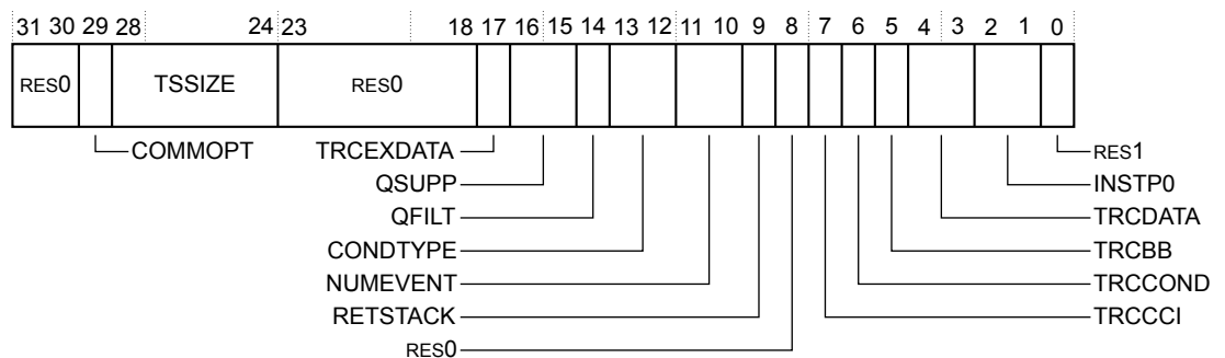
Figure B1-20 TRCIDR0 bit assignments
