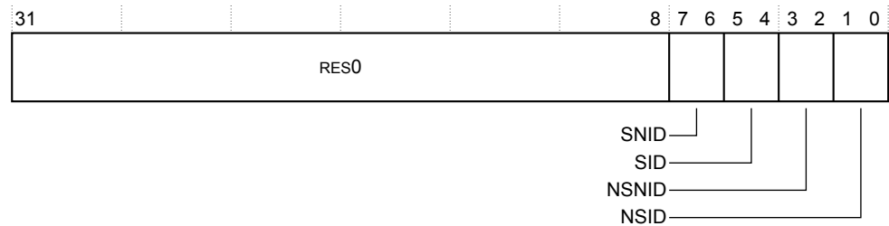
Figure B1-38 TRCAUTHSTATUS bit assignments
