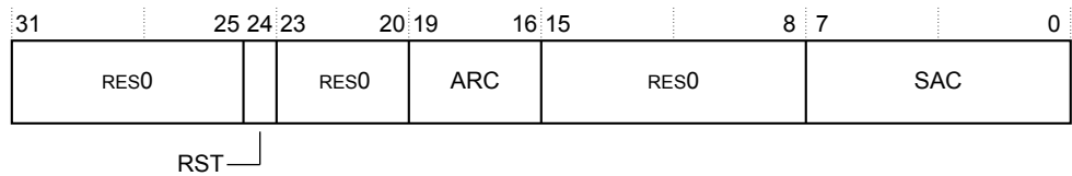
Figure B1-27 TRCSSCCR0 bit assignments
