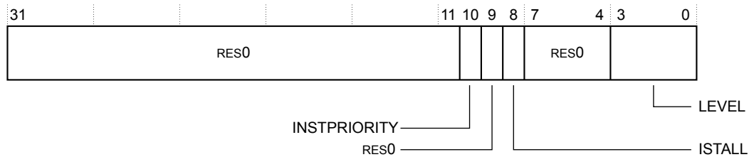
Figure B1-6 TRCSTALLCTLR bit assignments
