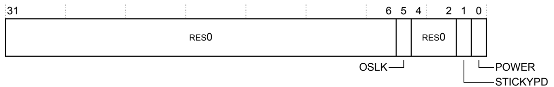
Figure B1-31 TRCPDSR bit assignments
