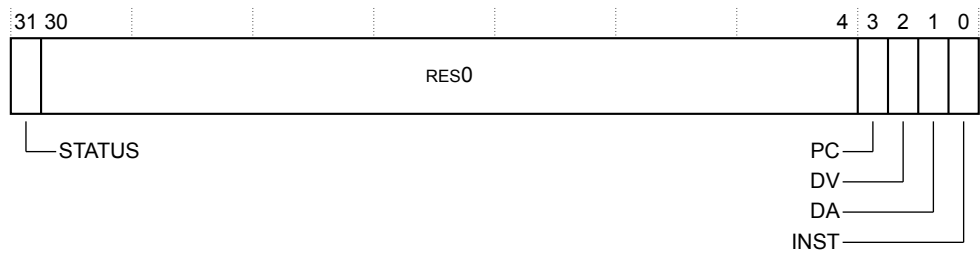
Figure B1-28 TRCSSCSR0 bit assignments
