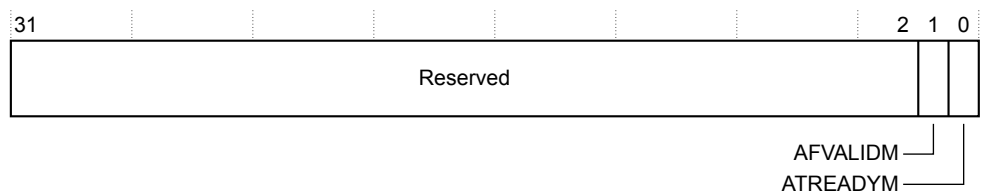
Figure B1-33 TRCITIATBINR bit assignments
