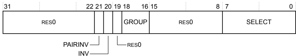
Figure B1-26 TRCRSCTLRn bit assignments
