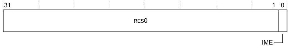
Figure B1-35 TRCITCTRL bit assignments
