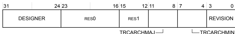
Figure B1-21 TRCIDR1 bit assignments
