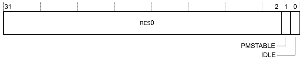
Figure B1-2 TRCSTATR bit assignments
