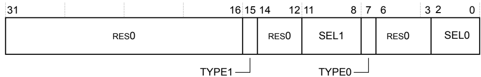
Figure B1-4 TRCEVENTCTL0R bit assignments
