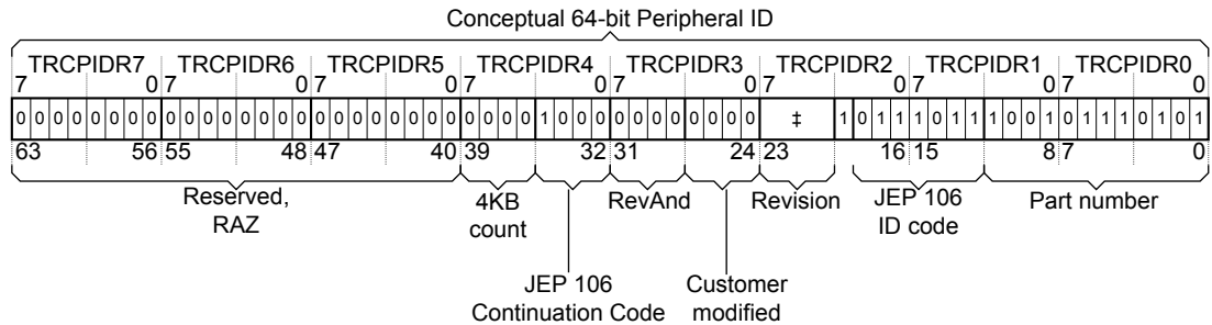
Figure B1-43 Peripheral ID fields
