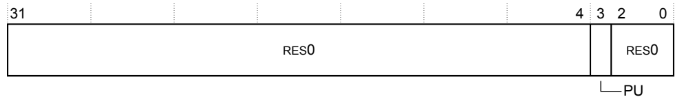
Figure B1-30 TRCPDCR bit assignments
