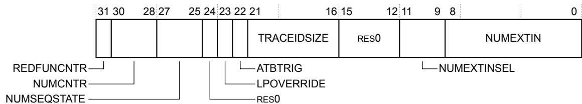
Figure B1-25 TRCIDR5 bit assignments
