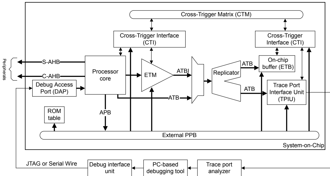
Figure A1-1 Example CoreSight system with ETM-M33
