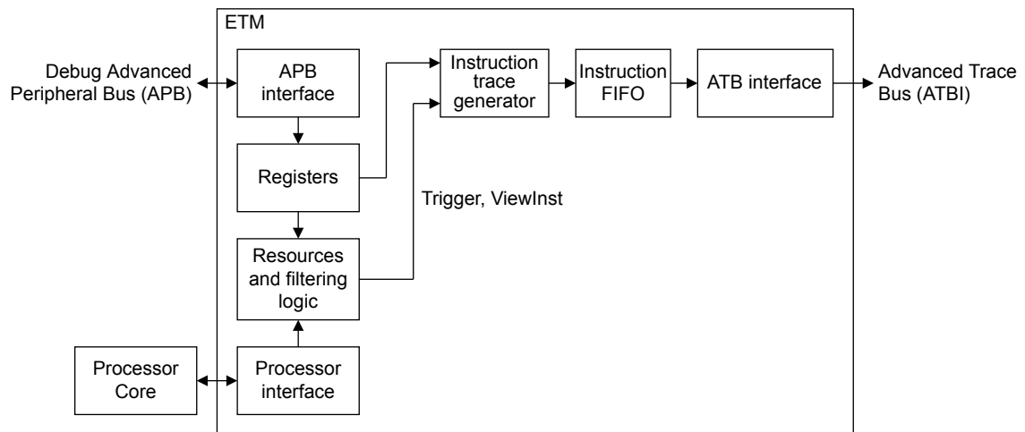
Figure A2-1 ETM-M33 block diagram
