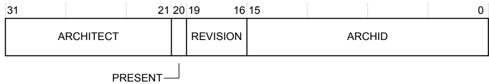
Figure B1-39 TRCDEVARCH bit assignments
