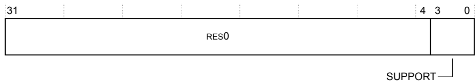
Figure B1-19 TRCIMSPEC0 bit assignments
