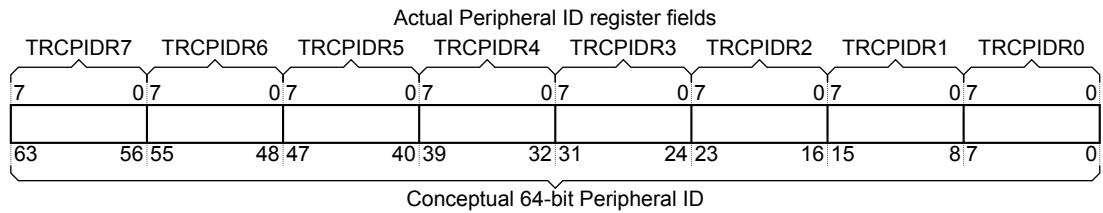
Figure B1-42 Mapping between TRCPIDR0-7 and the Peripheral ID value
