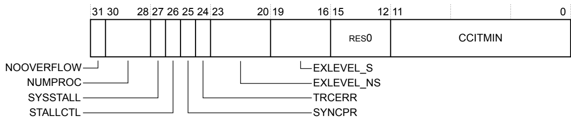
Figure B1-23 TRCIDR3 bit assignments
