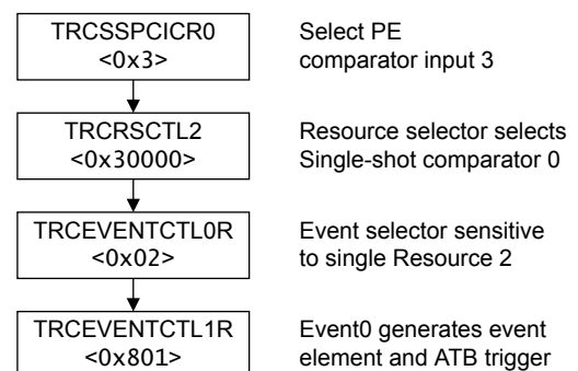
Figure A2-2 Trigger event resource selection
