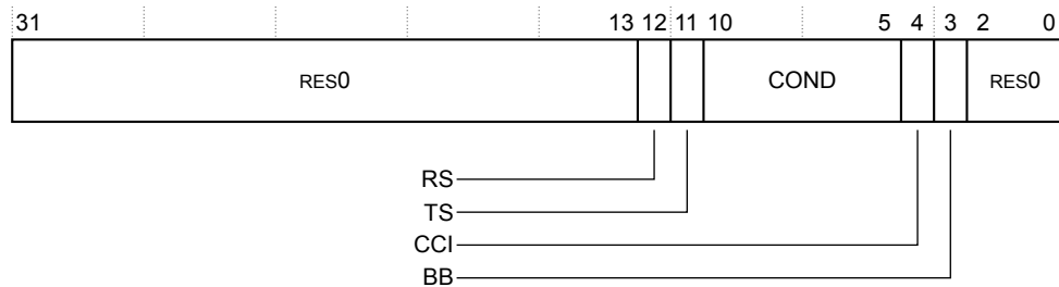
Figure B1-3 TRCCONFIGR bit assignments
