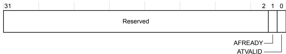
Figure B1-34 TRCITIATBOUTr bit assignments
