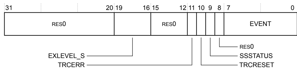
Figure B1-11 TRCVICTLR bit assignments
