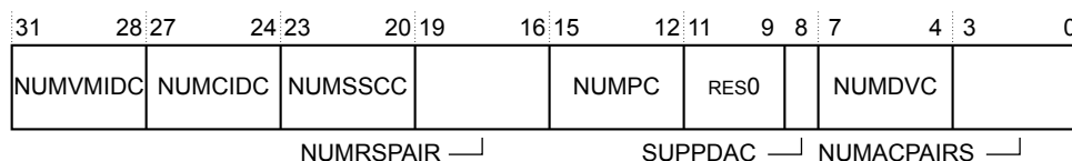
Figure B1-24 TRCIDR4 bit assignments
