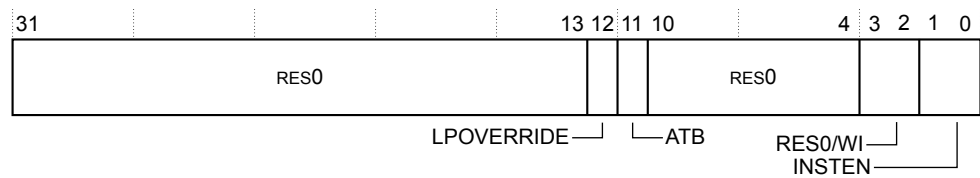
Figure B1-5 TRCEVENTCTL1R bit assignments
