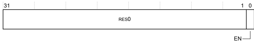
Figure B1-1 TRCPRGCTLR bit assignments
