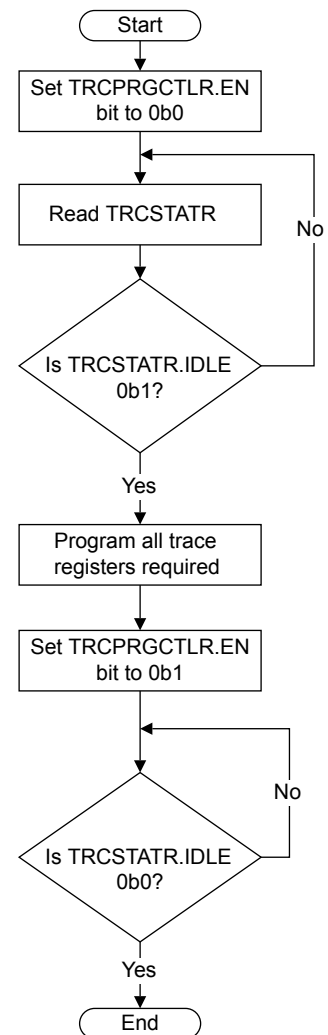
Figure A3-1 Programming ETM registers
