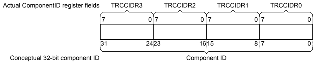
Figure B1-44 Mapping between TRCCIDR0-3 and the Component ID value
