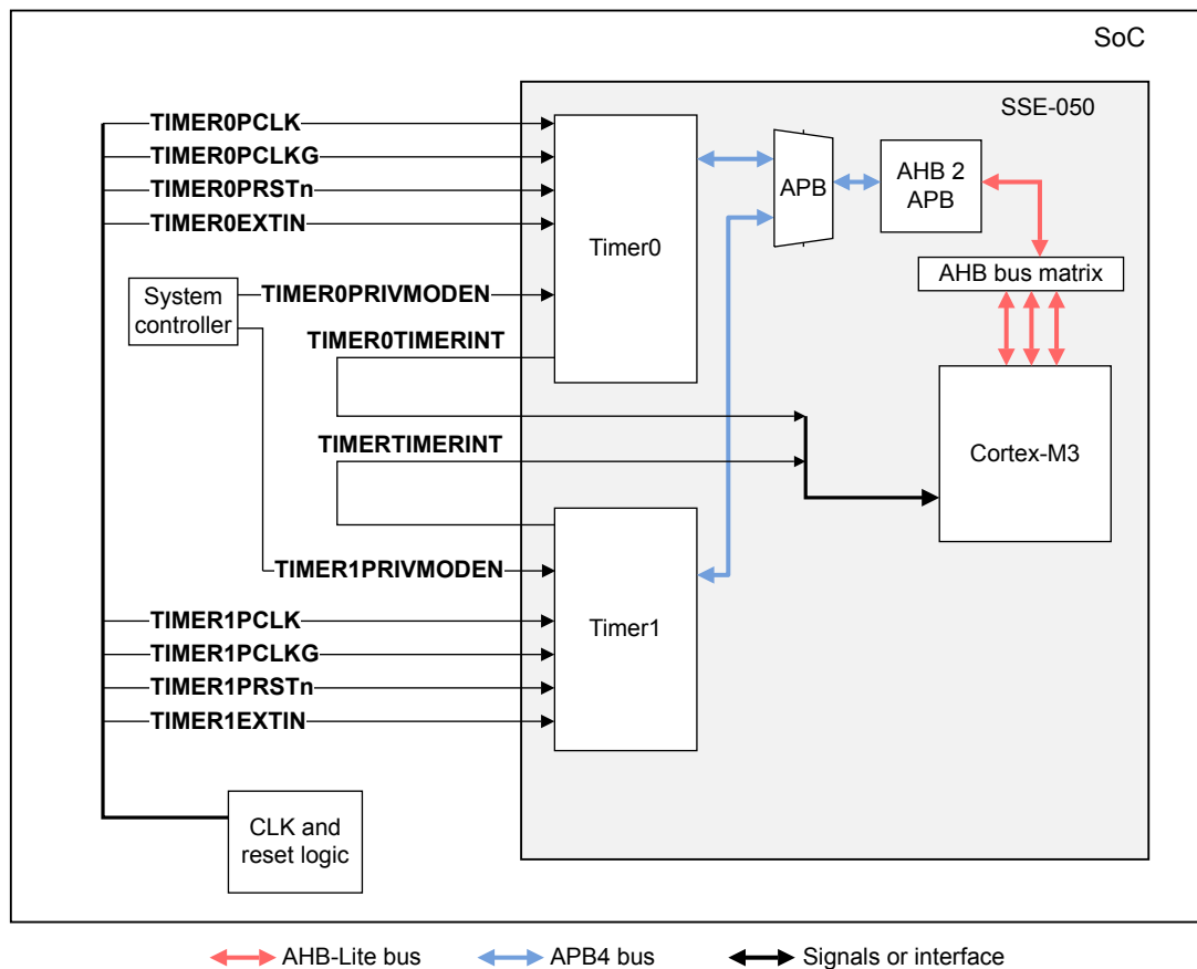
Figure 2-3 Timer interfaces
