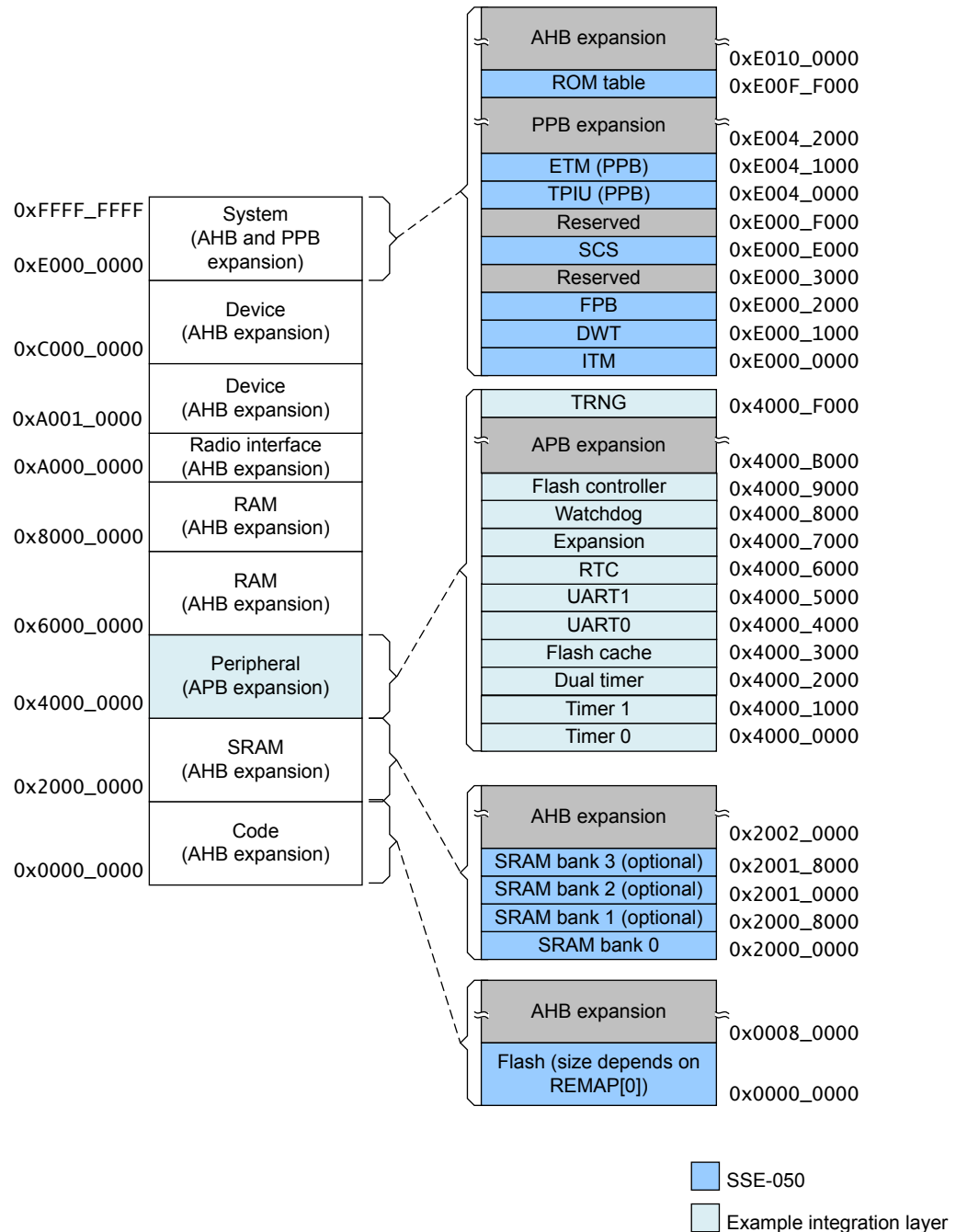
Figure 3-1 Top-level memory map
