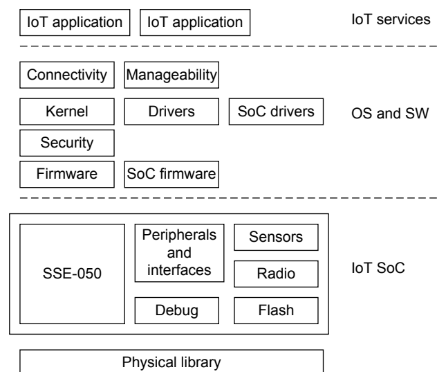
Figure 1-2 IoT endpoint HW and SW solution
