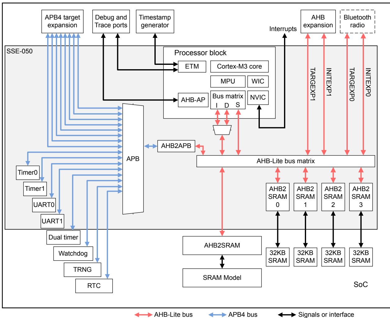
Figure 2-1 Bus interconnections
