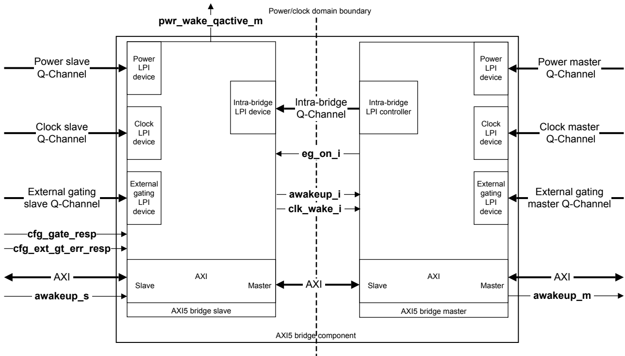
Figure 6-1 Bridge component interfaces
