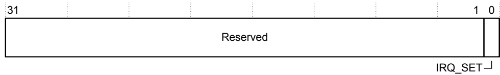
Figure 7-11 IRQ_SET bit assignments
