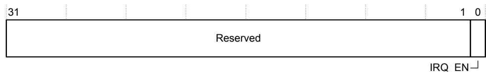
Figure 7-8 IRQ_EN bit assignments
