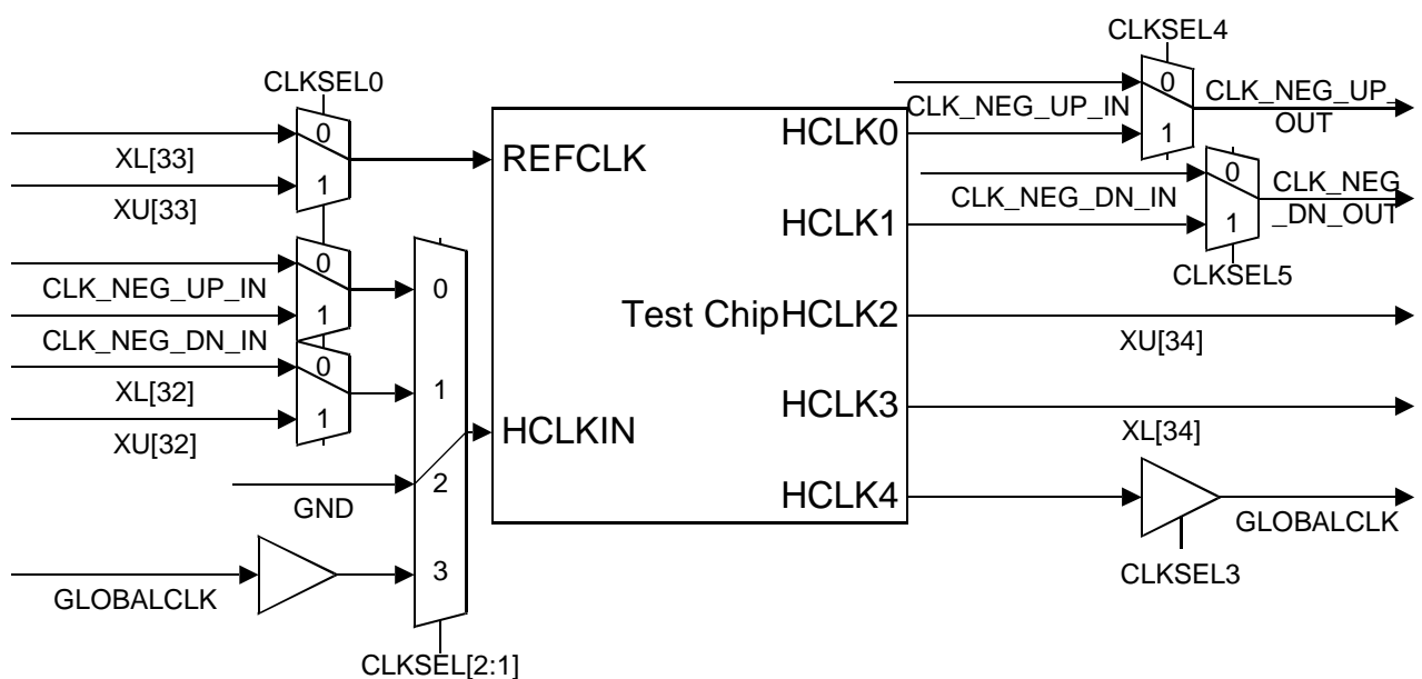
Figure 3-3 Core Tile clock routing
