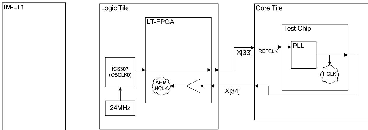
Figure 3-2 Clock architecture – HCLK
