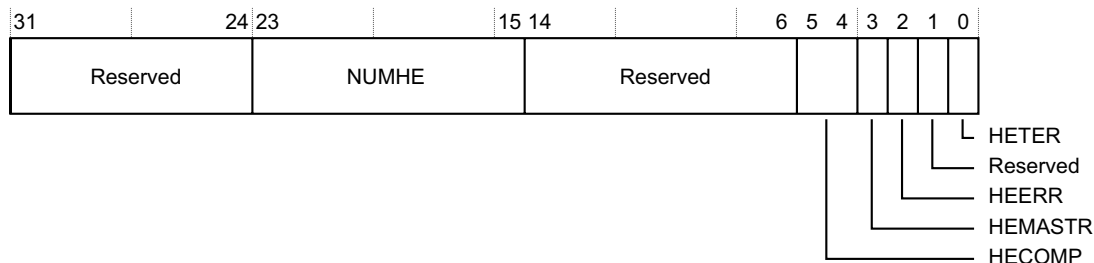
Figure 3-3 STMHEFEAT1R Register bit assignments
