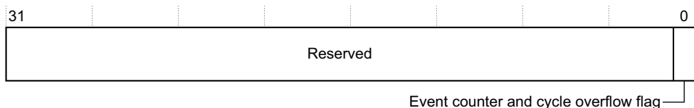
Figure 3-18 Overflow Flag Status Register bit assignments
