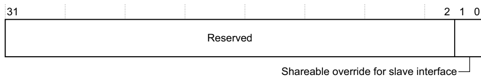
Figure 3-8 Shareable Override Register bit assignments
