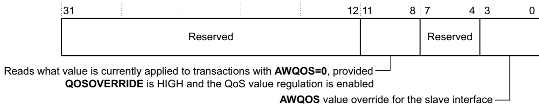
Figure 3-10 Write Channel QoS Value Override Register bit assignments
