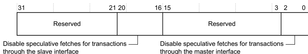
Figure 3-2 Speculation Control Register bit assignments
