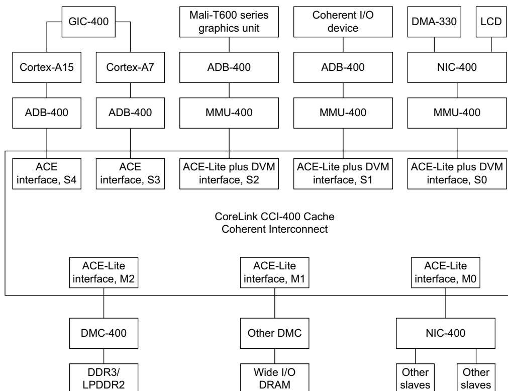
Figure 1-1 Example system with a CCI-400
