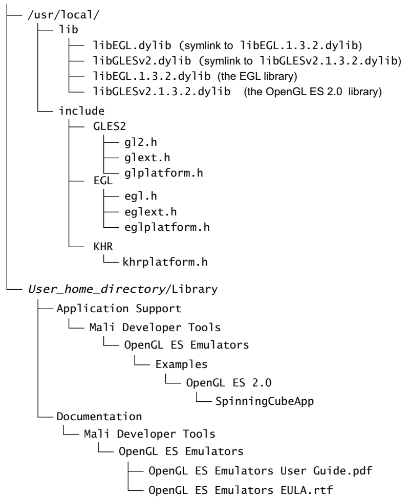
Figure 4-1 OpenGL ES emulator directory structure
