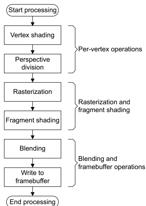
Figure 1-1 Graphics pipeline flow
