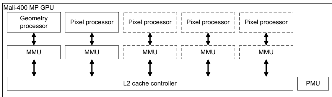
Figure 1-2 Mali-400 MP GPU
