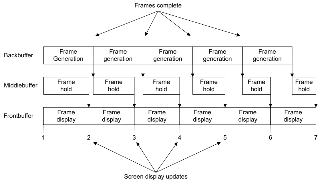
Figure 2-4 Screen updates with triple buffering and VSYNC
