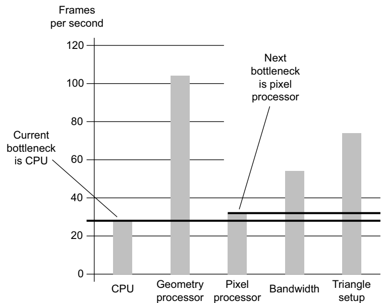
Figure 3-3 Frame rate limitations of different system elements
