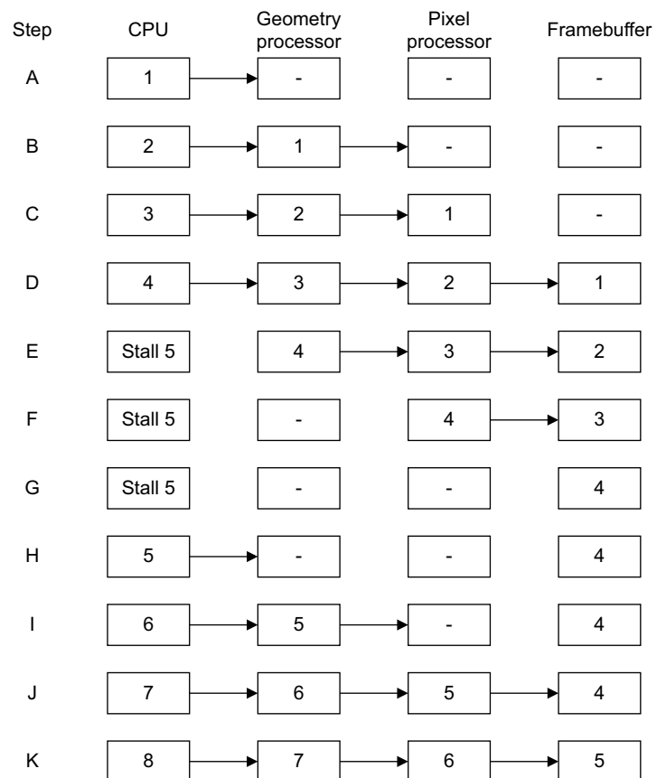
Figure 4-1 Graphics pipeline flow with stall
