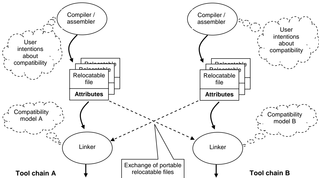
Figure 2-1, software development flows supported by build attributes
